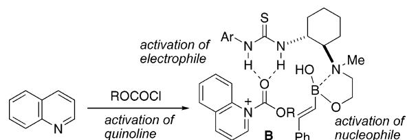
Figure 1. Concept of a newly designed thiourea catalyst.
